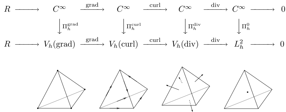
Fig. 5.1. Exact sequences, commutative diagrams and degrees of freedom for the finite element spaces in the lowest order case.
