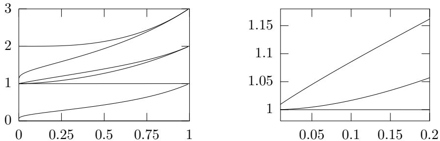
Figure 12: Two views of the smallest five generalized real eigenvalues, as calculated from (85) with D = 0 , using the solutions U_\lambda , given by (86).
