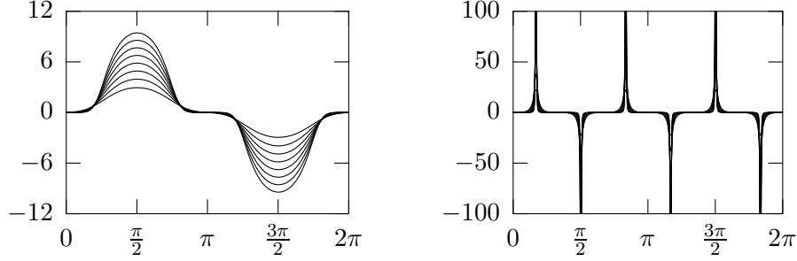
Figure 3: Left frame: normal boundary flux component \lambda \sinh(u_\lambda) for \lambda negative (smallest flux: \lambda \sim -.64 \times 10^{-1} , largest flux \lambda \sim -.56 \times 10^{-4} ). Right frame : normal boundary flux component \lambda \sinh(u_\lambda) for \lambda positive (smallest flux: \lambda \sim .85 \times 10^{-1} , largest flux \lambda \sim .75 \times 10^{-4} ). In both frames D = 1.5 .
