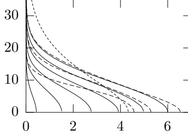
Figure 7: H^1(\Omega) -norms of solutions to (1), with D = 0 on the annulus, \Omega = B(0,1) \setminus \overline{B(0,1/2)} . Only primary bifurcations are plotted.
