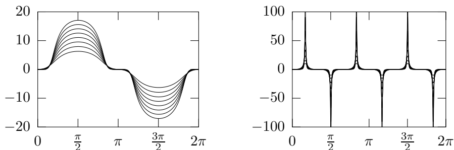
Figure 2: Left frame: normal boundary flux component \lambda \sinh(u_\lambda) for \lambda negative. Right frame : normal boundary flux component \lambda \sinh(u_\lambda) for \lambda positive. In both frames D = 2 .
