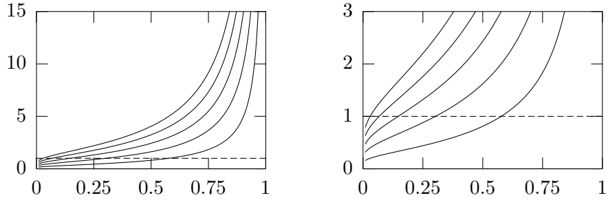
Figure 11: Two views of the smallest five generalized real eigenvalues, as calculated from (85) with D = -1 and U_\lambda in the form of the constant solution. We expect a bifurcation whenever a curve of generalized eigenvalues crosses \gamma = 1 . This expectation is confirmed by comparison with the bifurcation plot, shown in Figure 10.
