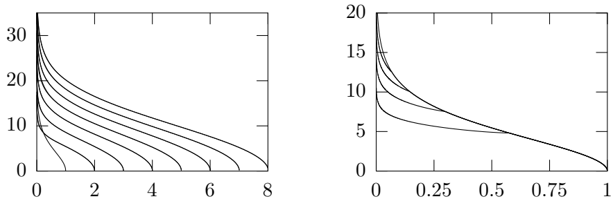
Figure 10: Two views of solutions to (1) for D = -1 on the unit ball. The left frame shows the first 8 primary bifurcations from the zero solution. The right frame shows the constant solution with its first 4 secondary bifurcations.
