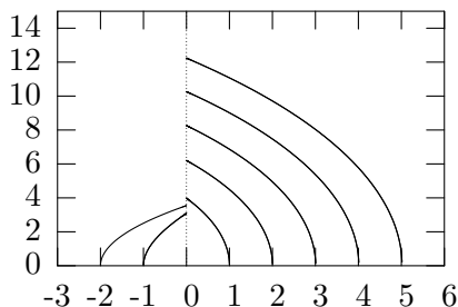
Figure 5: The H^1(\Omega) -norm of v_\lambda = \lambda^{1/2}u_\lambda as a function of \lambda for different solutions to (83), f(u) = u + u^3 .
