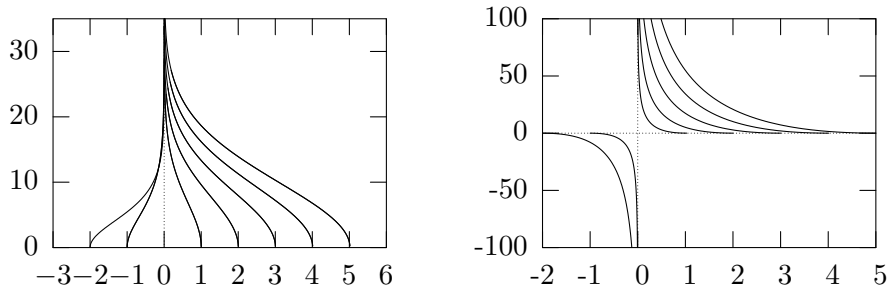
Figure 1: Left frame: H^1(\Omega) -norm as a function of \lambda for different solutions to (1). Right frame : energies E_\lambda for the same solutions.
