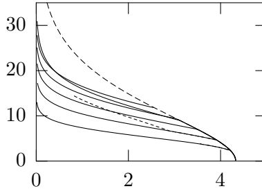
Figure 9: The radial solution, with a collection of secondary and, what appears to be, one tertiary bifurcation.
