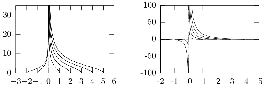
Figure 4: Left frame: the H^1(\Omega) -norm as a function of \lambda for different solutions to (83) with f(u) = u + u^3 . Right frame : the energies E_\lambda for the same solutions.
