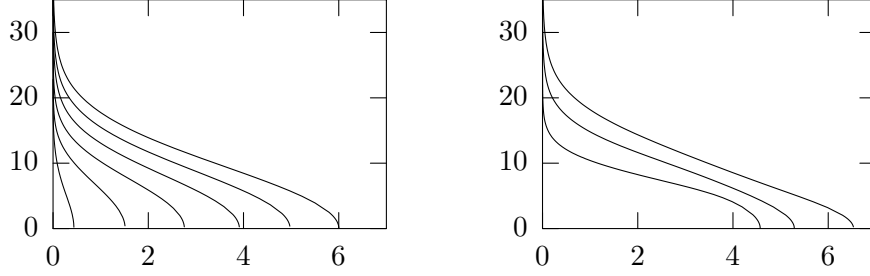
Figure 8: Primary bifurcations on the annulus. The left frame shows the H^1(\Omega) -norms associated with the (first 6) solutions we have designated class A. The right frame shows the H^1(\Omega) -norms associated with the (first 3) solutions we have designated class B.
