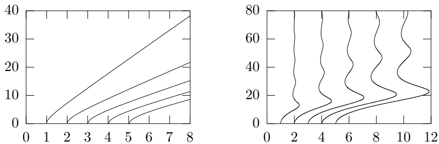
Figure 6: The H^1(\Omega) -norm of “the first” five solutions to (83) with f(u) = \arctan(u) (left frame) and f(u) = \frac{1}{2}(u + \sin(u)) (right frame). In both cases D = 0 .
