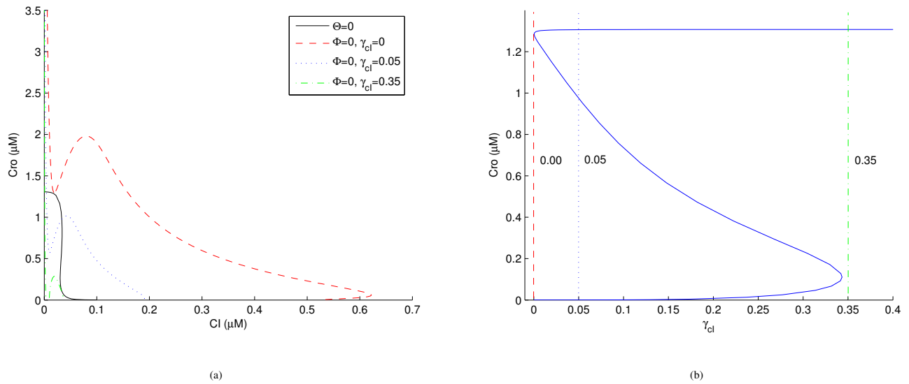
Fig. 2. A. Nullclines for \Theta = 0 (black solid) and \Phi = 0 with \gamma_{cI} = 0 \text{ min}^{-1} (red dash), \gamma_{cI} = 0.05 \text{ min}^{-1} (blue dots) and \gamma_{cI} = 0.35 \text{ min}^{-1} (green dash-dot). B. Bifurcation diagram of \gamma_{cI} versus [Cro].
