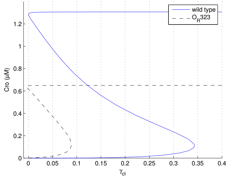
Fig. 3. Bifurcation diagrams for wild type and O_{R323} . The concentration of Cro is graphed as a function of \gamma_{cl} . The blue solid curve represents the wild type phase, while the black dashed curve represents the mutant.
