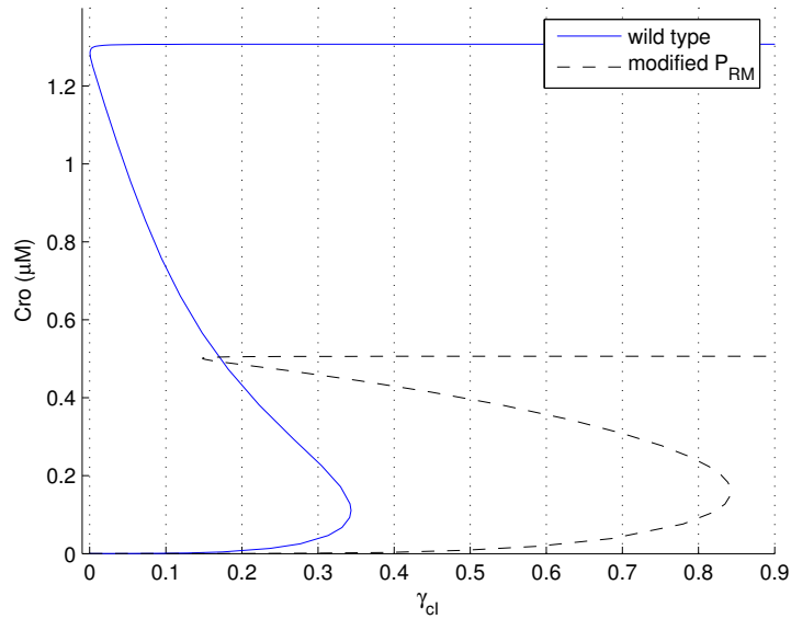
Fig. 4. Bifurcation diagram of wild type vs. a phage with mutated P_{RM} binding site which resulted in having P_{RM} = -12.5 kcal/mol, \phi = 4.5/.35 , and P_R = -10.5 kcal/mol. For comparison, the wild type values were P_{RM} = -11.5 kcal/mol, \phi = 4.29/.35 , and P_R = -12.5 kcal/mol.
