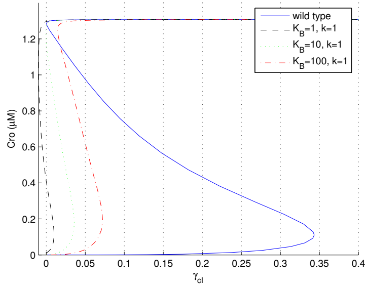
Fig. 6. Results from eliminating positive control ( \phi = 1 ) with values of \beta = 1 (black dashed curve), \beta = 10 (green dotted curve) and \beta = 100 (red dash-dot curve). We graph concentration of Cro as a function of \gamma_{cl} .
