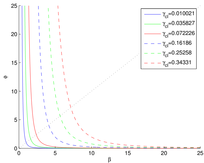
Fig. 7. Level curves of the induction value \gamma_* as a function of both \beta and \phi . Here \beta > 1 represents K_B -cooperativity and \phi > 1 represents k -cooperativity.
