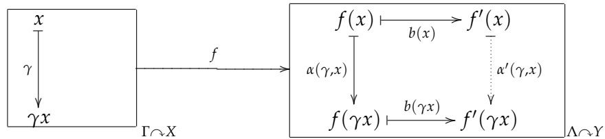
FIGURE 2. If f, f' differ only by multiples of \Lambda , then their corresponding cocycles \alpha, \alpha' are cohomologous.
