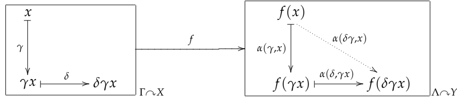
FIGURE 1. The cocycle \alpha corresponds to f .
