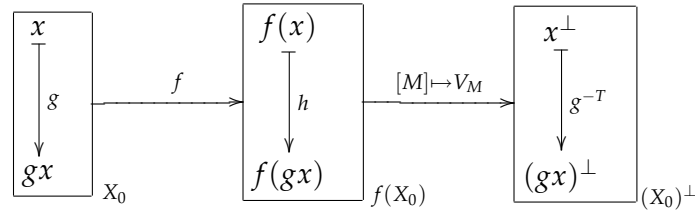
FIGURE 1. We have forced that an element of the form h = ag^{-T} witnesses that f(x) \cong_{n,p}^{n-k} f(gx) .
