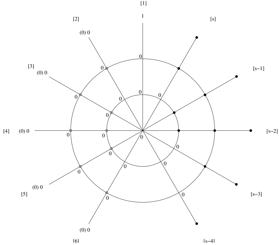
Figure 3: A circular 2-ring network, with vertices numbered in brackets
