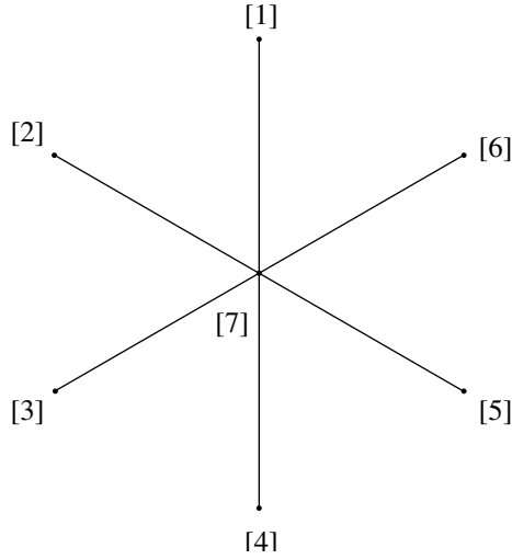
Figure 1: A 6-star graph
