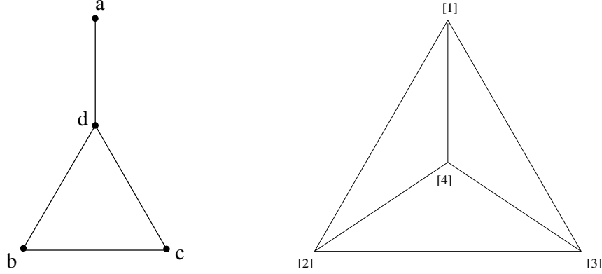
Figure 2: The capped delta graph (left), with conductivities labelled and; a complete graph (right) of 3 boundary nodes and one interior node
