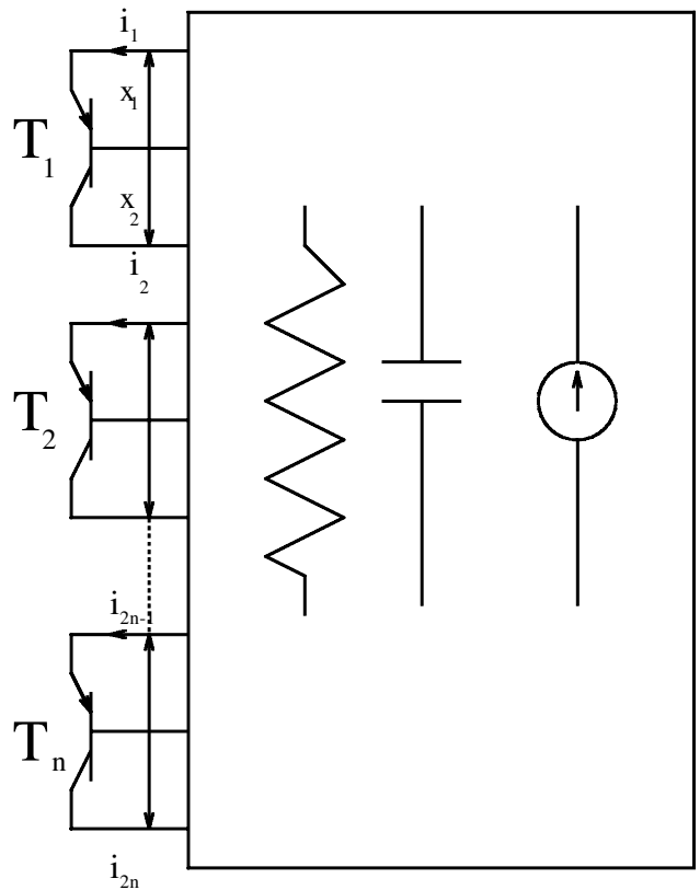
Figure 2. Transistor network.
