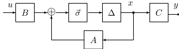
Figure 1: Block Diagram of Recurrent Net
