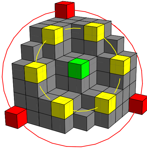
FIGURE 1. A totally symmetric plane partition with largest part 7. The yellow cubes form an orbit of length 6 (corresponding to all permutations of (2, 4, 6) ), the red cubes an orbit of length 3 (all permutations of (1, 1, 7) ), and the green cube on location (4, 4, 4) represents an orbit of length 1.
