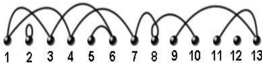
FIGURE 1. A tangled-diagram over 13 vertices.
